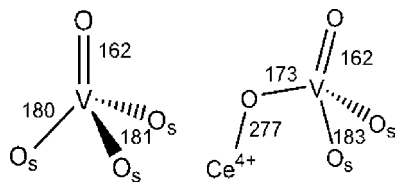
Figure 3. VO and VO 2 species on the defect-free CeO 2 (111) surface with bond distances in picometers.
